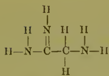
Methyluramin (p. 22).
